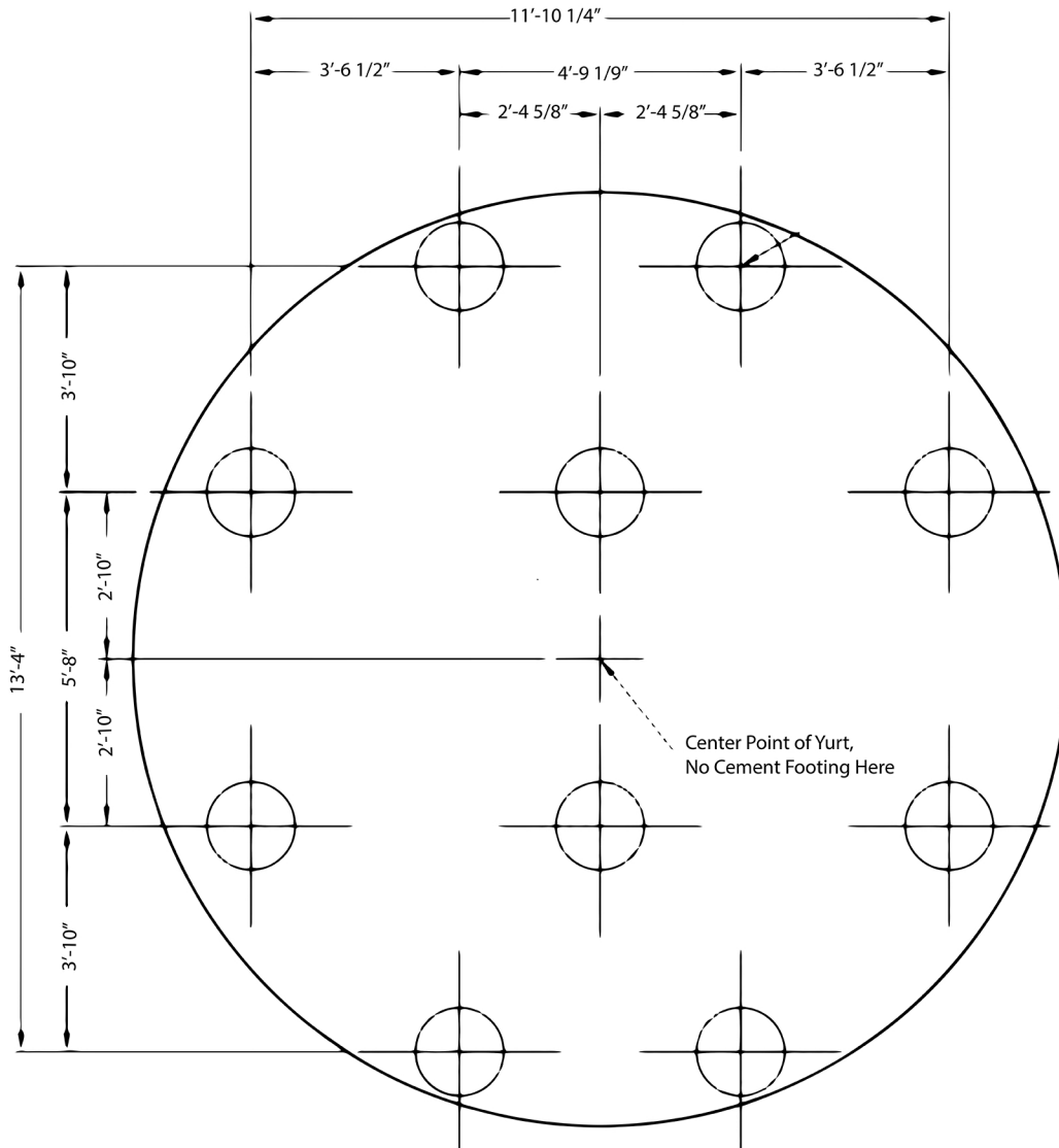
Footing Layout
